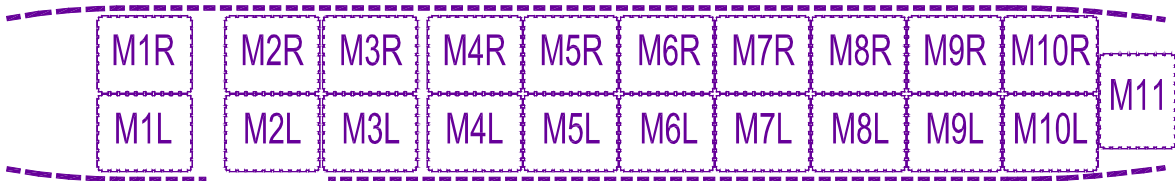
CONFIGURATION B 20 ULD's 108" X 88" SIDE BY SIDE 1 ULD 88" X 108" SINGLE ROW
