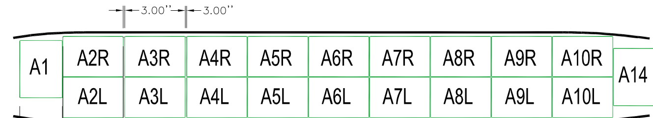
CONFIGURATION A 18 ULD's 125" X 88" SIDE BY SIDE 2 ULD 88" X 125" SINGLE ROW
