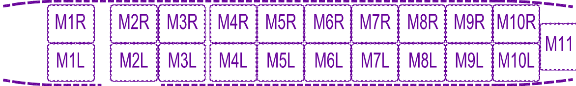
CONFIGURATION B 20 ULD's 108" X 88" SIDE BY SIDE 1 ULD 88" X 108" SINGLE ROW
