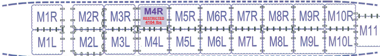
Configuration B (Purple) 20 - 108x88, 1 - 88x108 M4R - MAX WEIGHT 4104 lbs
