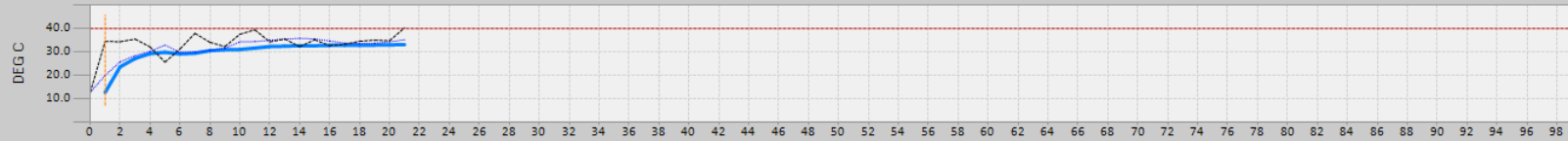
(EGT_CRZ_DEV_CV) - EGT Cruise Deviation 30 point average -- N371CM-2 -- 695546 CRUISE CHARTING
